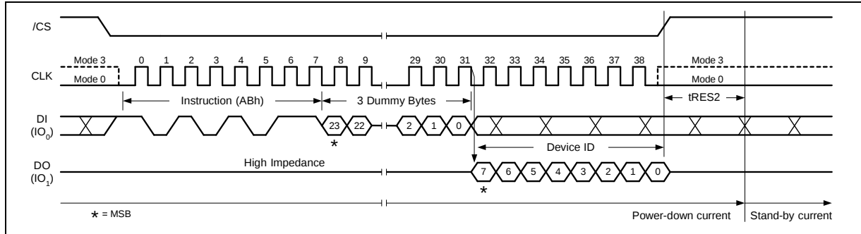
Figure 38c. Release Power-down / Device ID Instruction (SPI Mode)
