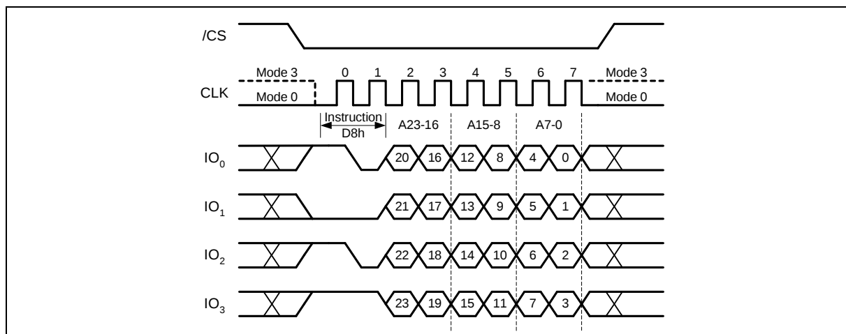
Figure 33b. 64KB Block Erase Instruction (QPI Mode) 32-Bit Address is required when the device is operating in 4-Byte Address Mode
